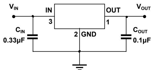
Conventional Circuit
