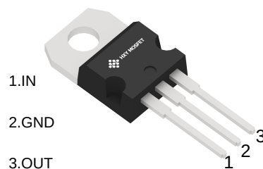
TO-220S
