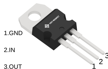
TO-220S
