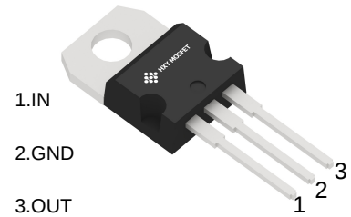
TO-220S
