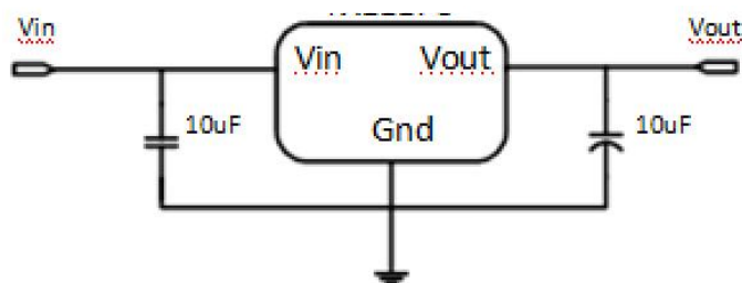
Application circuit of TLV1117-xxIDCYR fixed version
