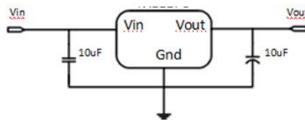
Application circuit of TLV1117-xxIDCYR fixed version
