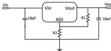
Application Circuit of TLV1117-ADJIDCYR
