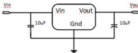
Application circuit of REG1117-xx/2K5 fixed version
