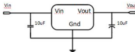
Application circuit of LM1117IMP-xx/NOPB fixed version
