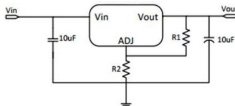
Application Circuit of LD1117SxxCTR
