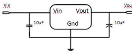
Application circuit of LD1117SxxCTR fixed version
