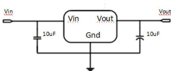
Application circuit of LD1117S fixed version
