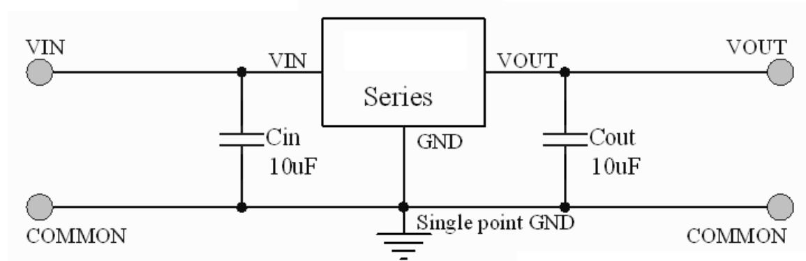
Application circuit of AMS1117-xx fixed version
