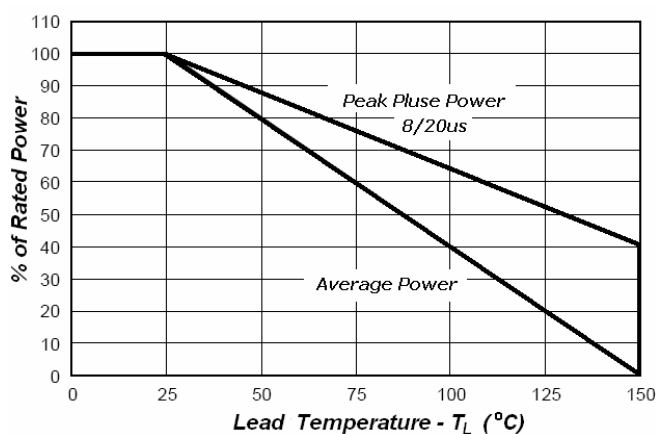
Fig 2. Power Derating
