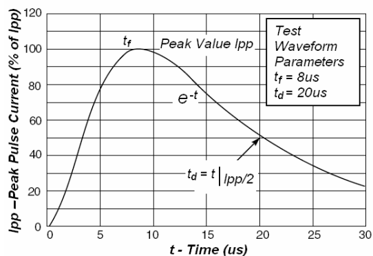
Fig 1. Pulse Waveform
