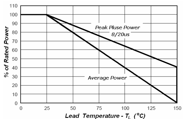
Fig 2. Power Derating
