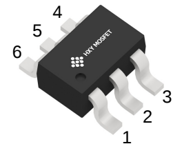
SOT-23-6L (TSOP-6-1.5mm)
