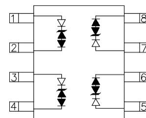
SOP-8 (SO-8)
