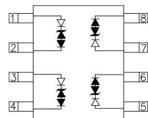
SOP-8 (SOIC-8)
