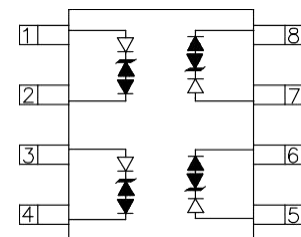
SOP-8 (SO-8)
