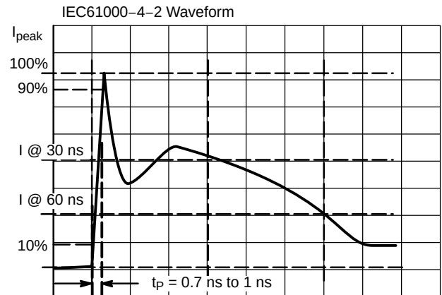
Figure 1. IEC61000-4-2 Spec
