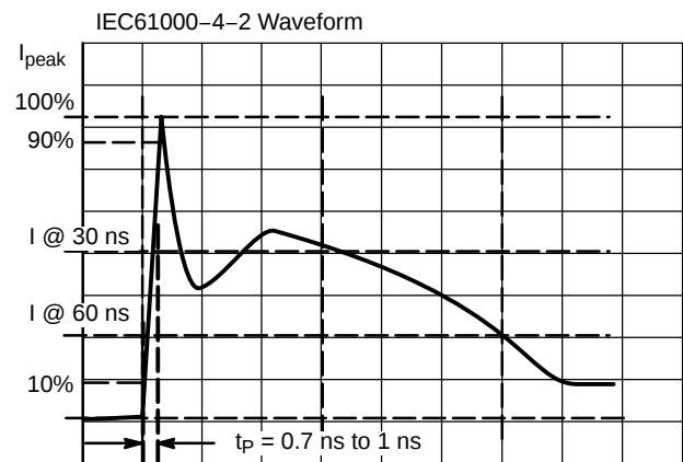
Figure 1. IEC61000-4-2 Spec
