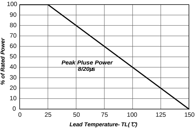
Fig2.Power Derating
