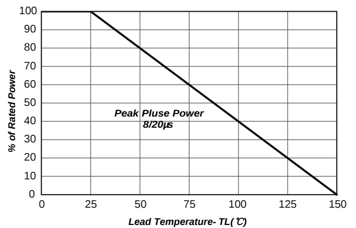
Fig2. Power Derating
