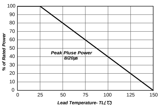
Fig2.Power Derating
