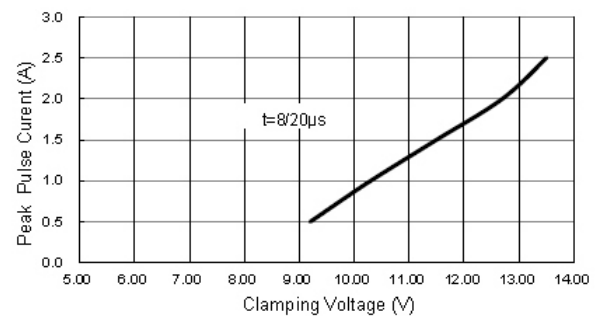
Fig 6 Clamping Voltage vs Peak Pulse Current
