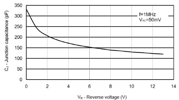
Capacitance vs. Reverse voltage
