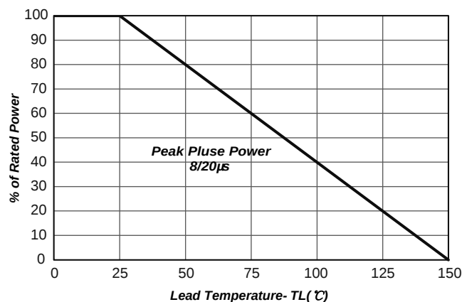
Fig2. Power Derating
