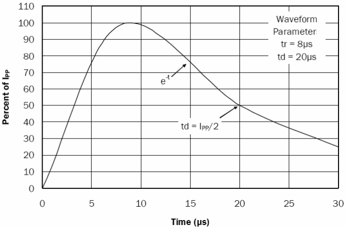
Fig.3 Waveform
