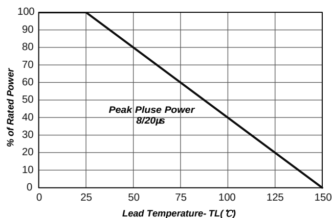
Fig2. Power Derating
