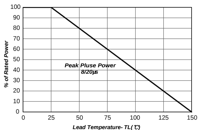
Fig2. Power Derating
