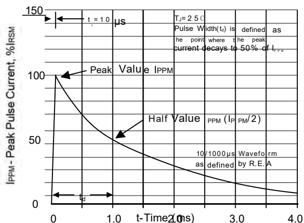
Figure 3. Pulse Waveform
