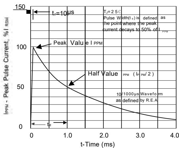
Figure 3. Pulse Waveform
