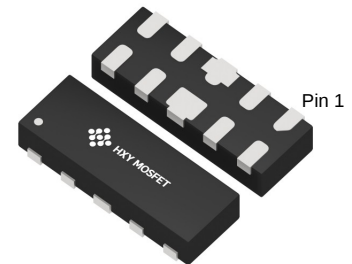
DFN2510-10L (DFN2510-10)
