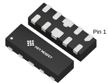
DFN2510-10L (DFN2510D-10))
