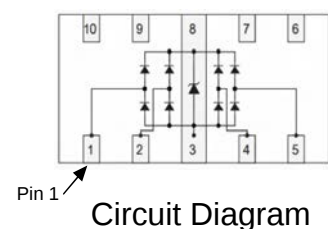
DFN2510-10L (DFN-10L(1x2.5))
