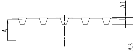
Side Vlew
