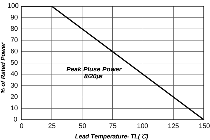
Fig2.Power Derating Curve
