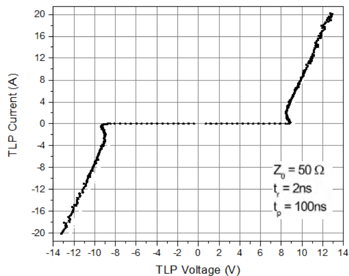
Fig1.TLP Measurement
