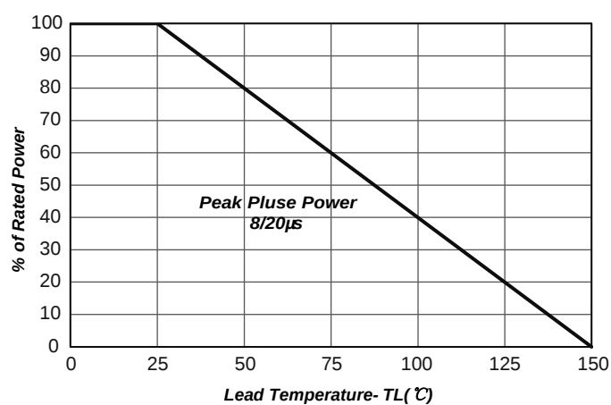
Fig3.Power Derating Curve
