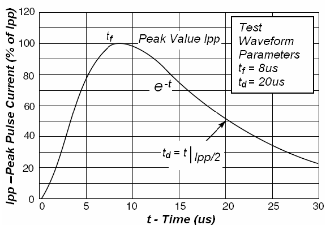
Fig2. Pulse Waveform
