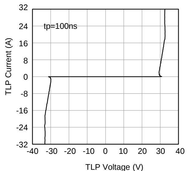
Fig 4. TLP Measurement
