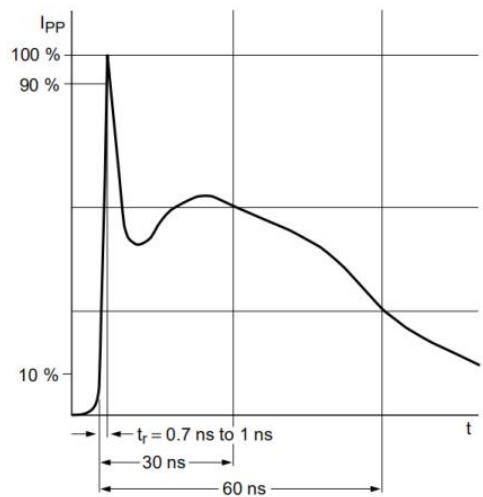
IEC61000-4-2 Waveform
