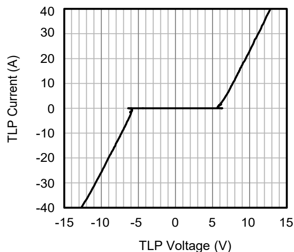
Fig4. TLP Measurement
