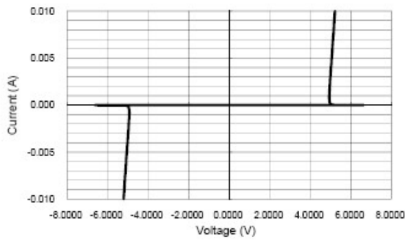
Fig 3 Voltage Sweeping
