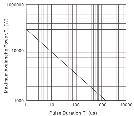
Fig. 6 - Maximum Avalanche Power Curve
