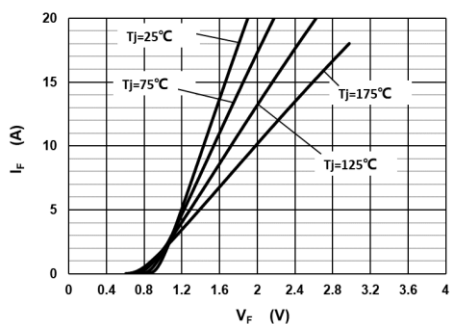
Fig 1: Forward Characteristics
