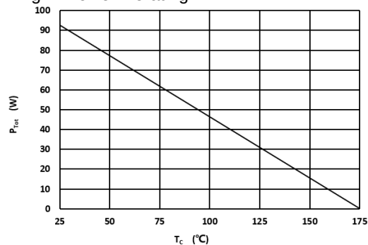
Fig 4: Power Derating
