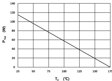
Fig 4: Power Derating
