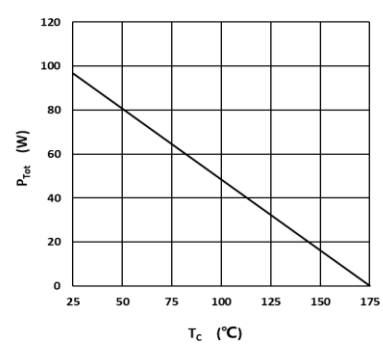
Fig 4: Power Derating
