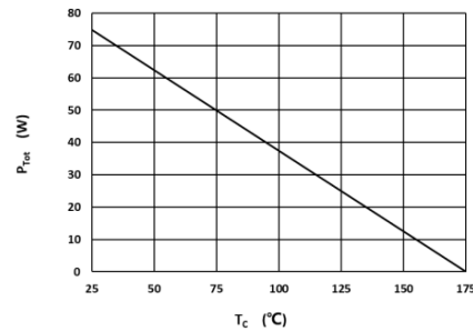
Fig 4: Power Derating
