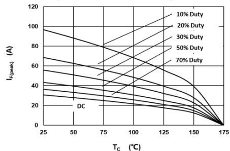
Fig 3: Current Derating
