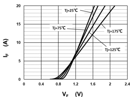
Fig 1: Forward Characteristics
