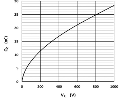
Fig 6: Reverse Charge vs. Reverse Voltage
