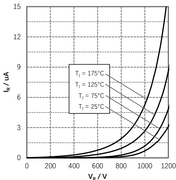
Figure 2. Reverse Characteristics
