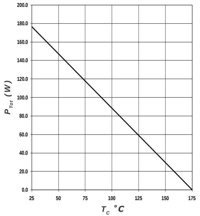
Figure 4. Power Derating
