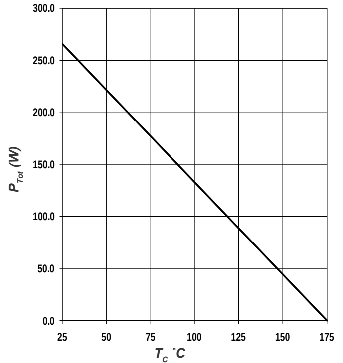
Figure 4. Power Derating
